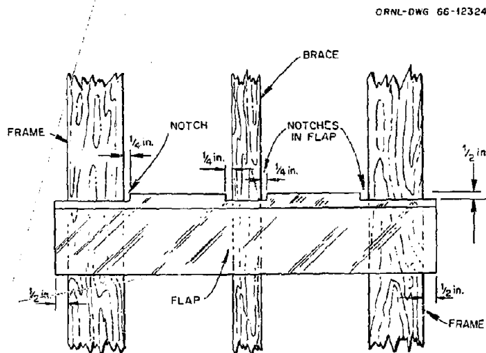
Fig. B-6. Size of notches in flaps
